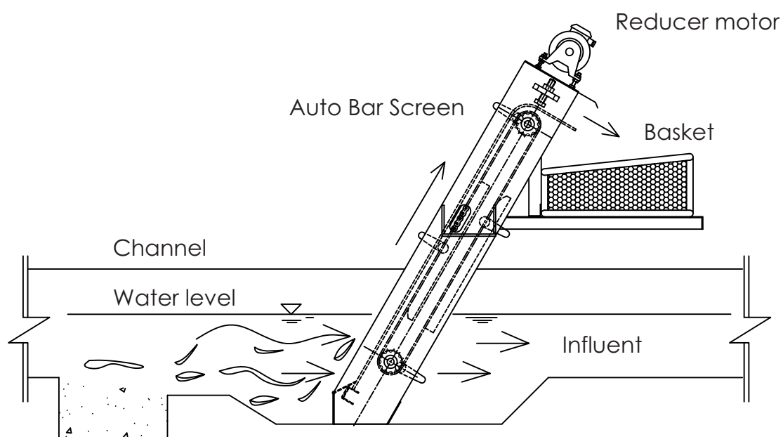
Schematic of Auto bar screen
